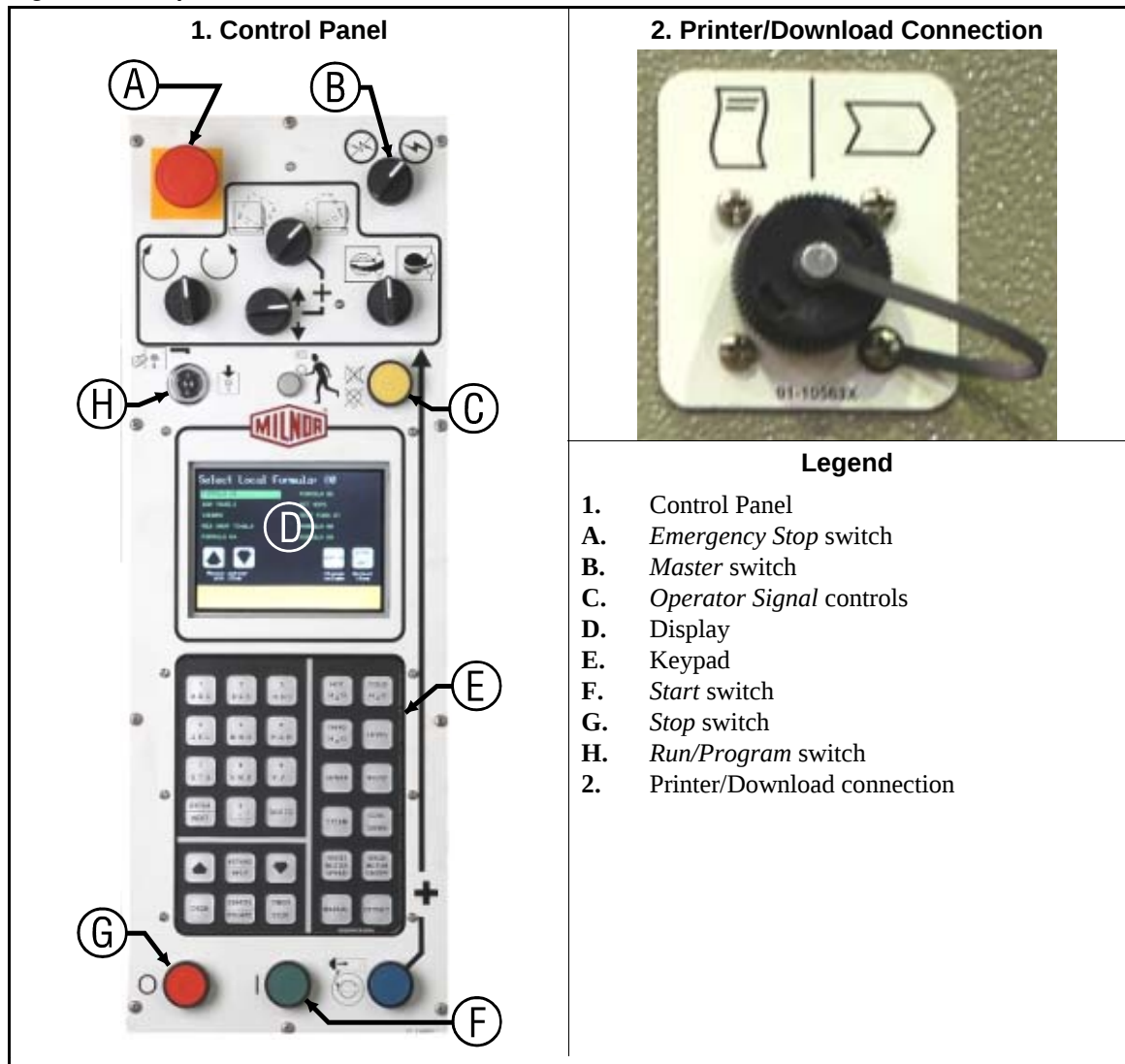
Figure 2: Microprocessor Interface Controls
